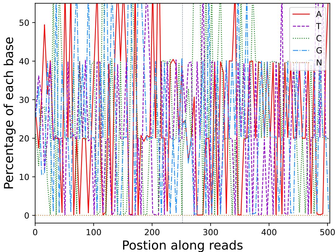
Base percentage along reads (R10304)
